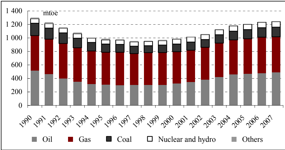
Figure 2.1. Primary Energy Supply, mtoe by Source Fuel (1990-2006)
